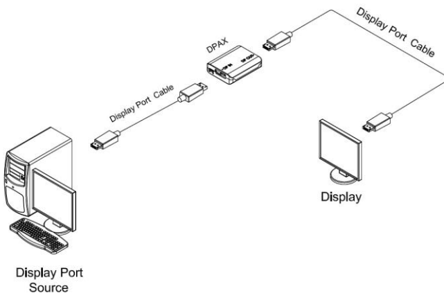
Figure 1 – Overall Connection of DPAX
